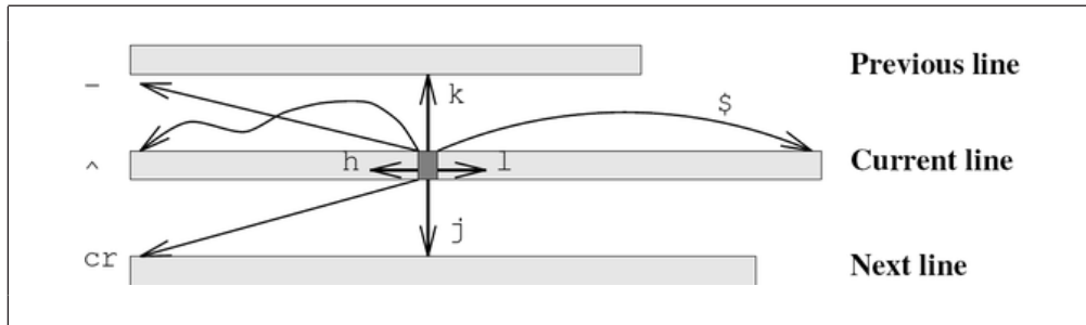
FIGURE 3 Cursor Movement
